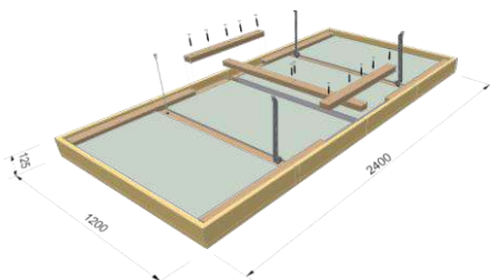
HERADESIGN® Sonic Element 2400 x 1200
